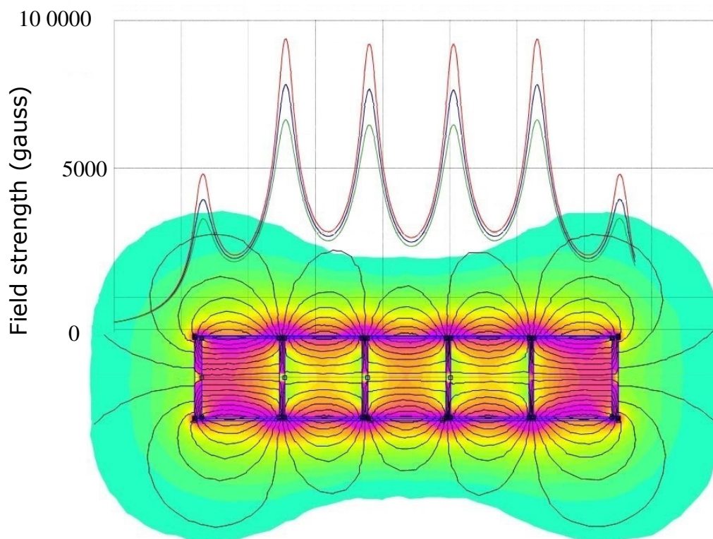
Magnetic bar Ø23 mm (GSN-42) in extractor tube Ø25 mm
